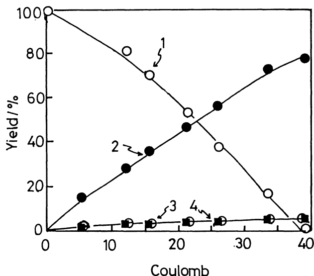
Fig. 1. Correlations of product yields with the electricity passed on electrochemical oxidation of 1 in CH 3 CN/CH 3 OH under argon.
